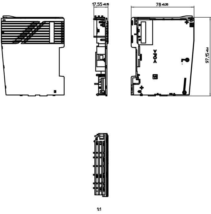
2ME-IO-S 24 COUPLER-HOUSING-R
