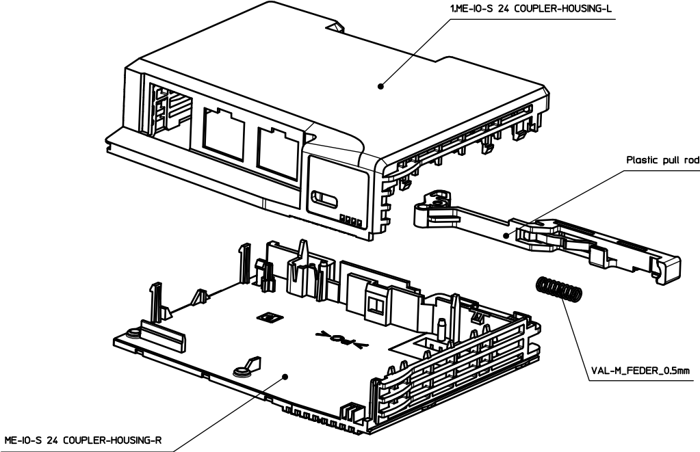
ME-IO-S 24 COUPLER-HOUSING-R
