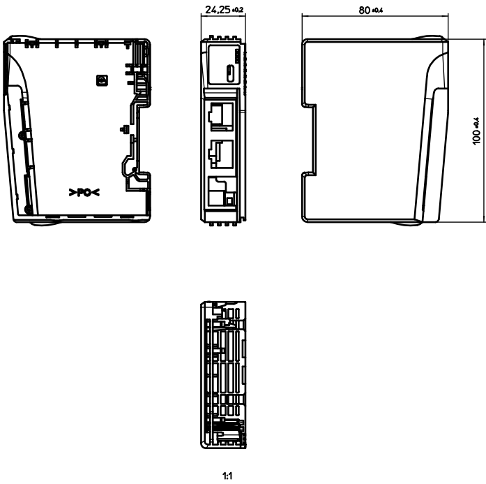
1ME-IO-S 24 COUPLER-HOUSING-L
